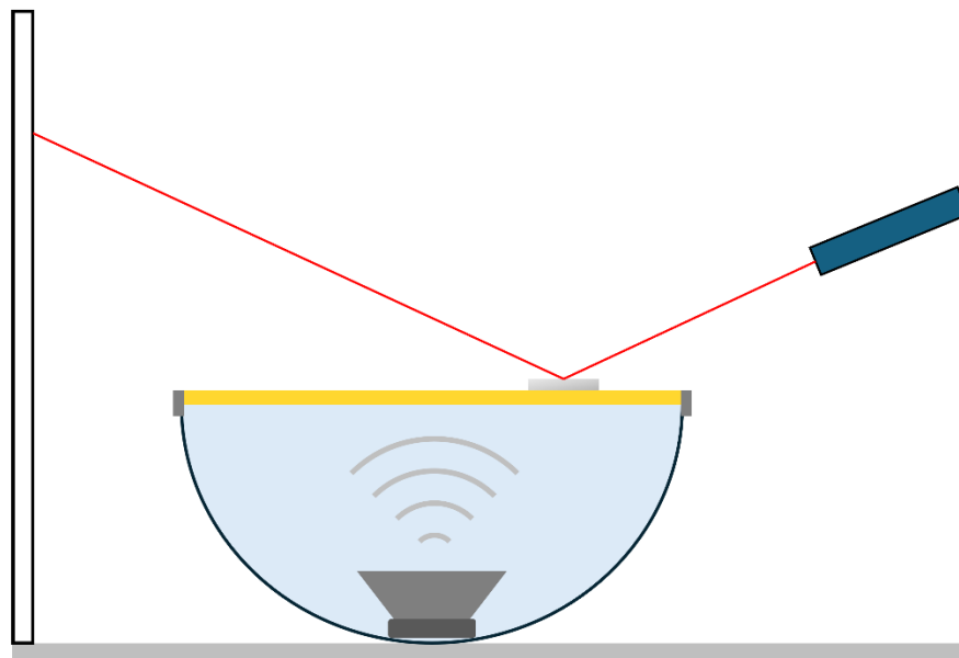
Schematic overview of the set up for Sound Visualisation.
